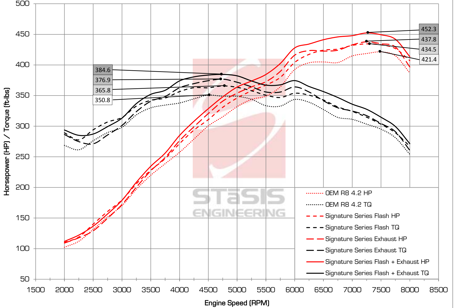
STāSIS Engineering R8 4.2 Exhaust/ECU Flash Comparison - Crankshaft Power
