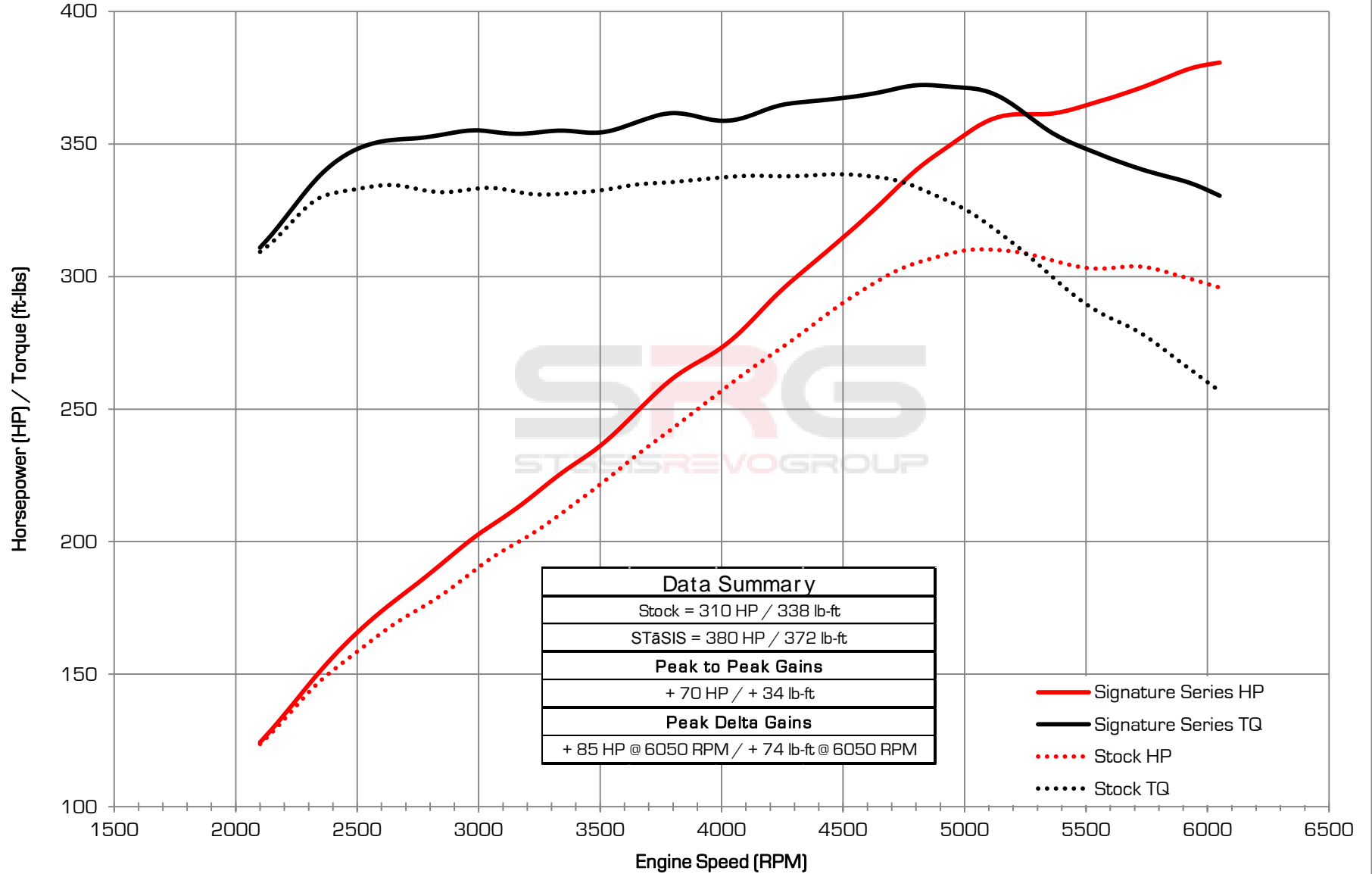
2012 A7 3.0T ECU Flash Comparison- Crankshaft Power
